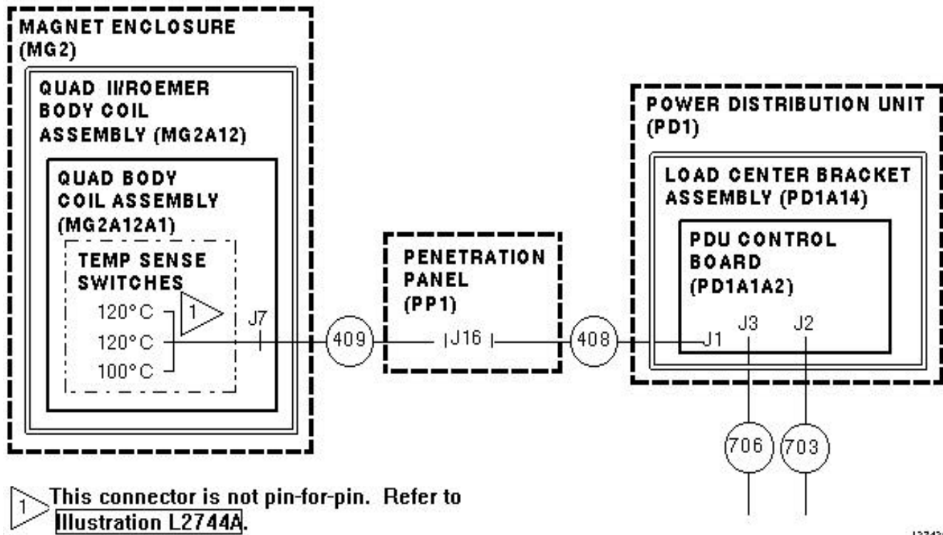
ILLUSTRATION L2742A COMPACT PDU OVERTEMPERATURE MONITORING INTERCONNECT
