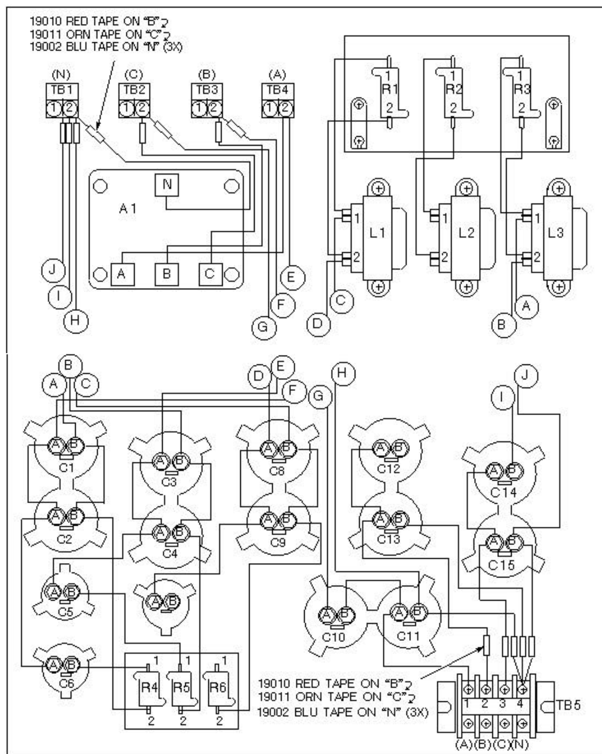
ILLUSTRATION L4796A FILTER COMP. LOCATIONS COMPACT PDU MODELS 46-317099P8 THROUGH P22
