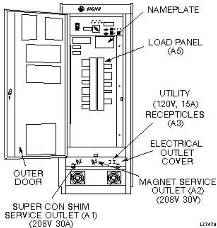
ILLUSTRATION L2747A FRONT PANEL AND LOAD PANEL COMPONENT LOCATIONS
