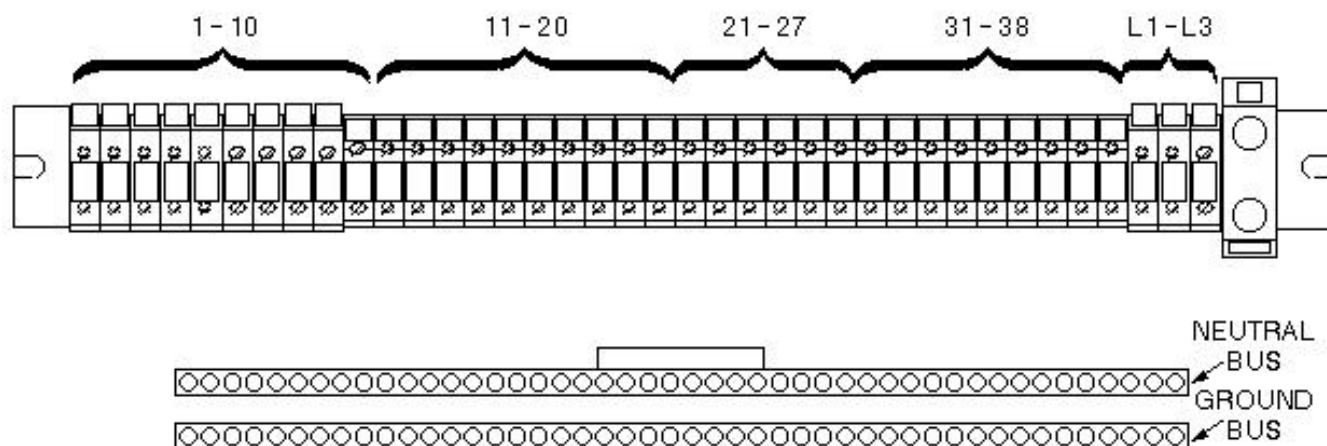
ILLUSTRATION L4795A TB10 (A2) AND BUS BARS MODELS 46-317099P8 THROUGH P22
