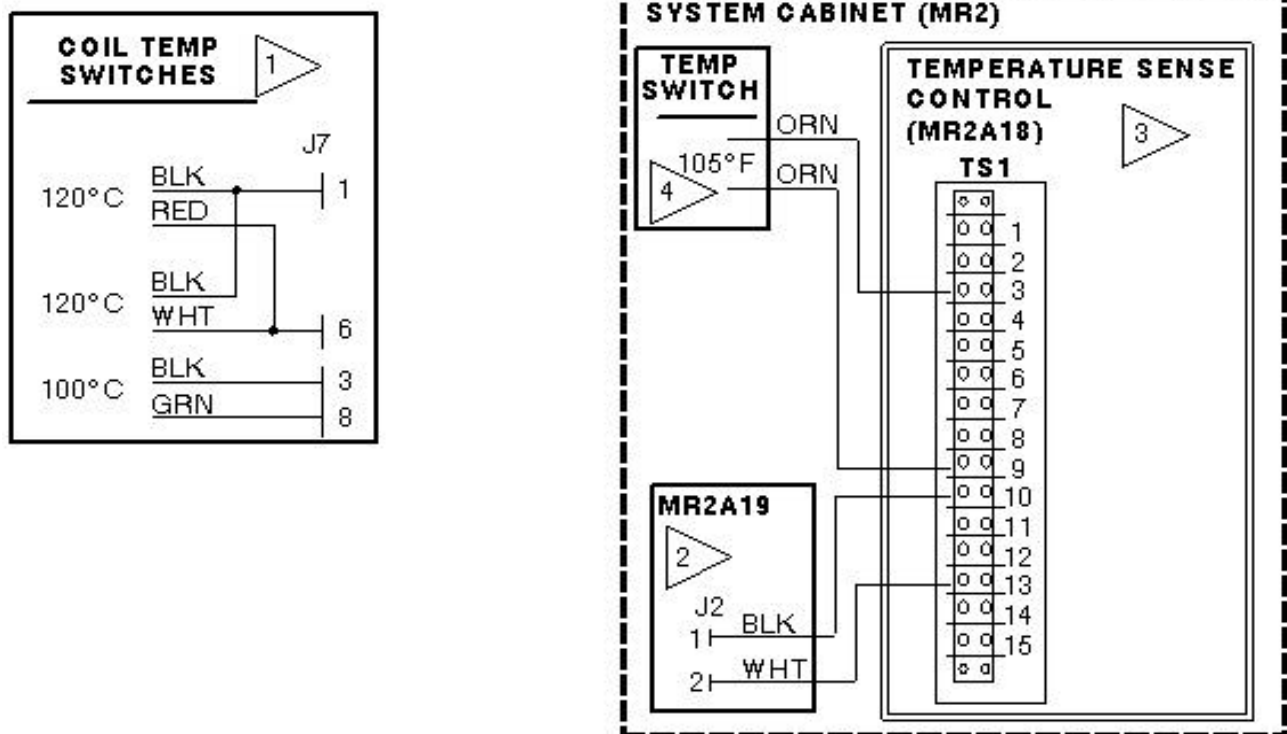
ILLUSTRATION L2744A COIL AND SYSTEM CABINET TEMPERATURE SWITCHES
