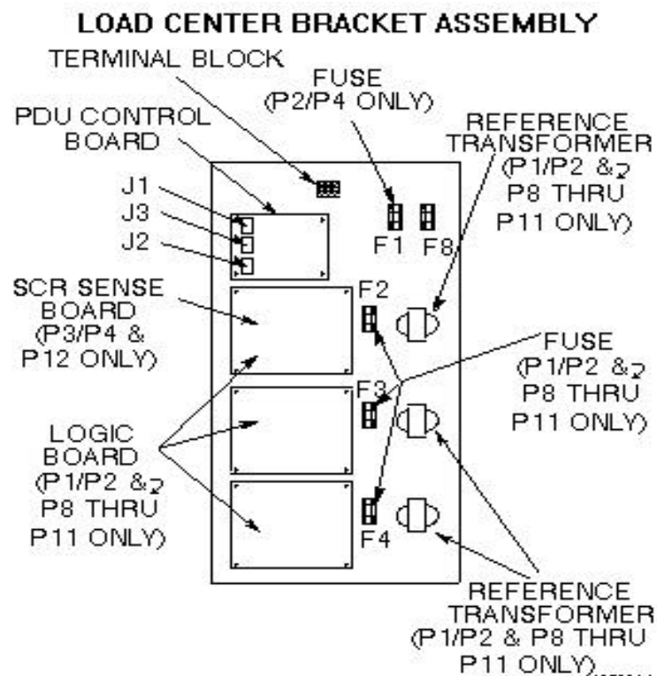
ILLUSTRATION L2722A LOAD CTR BRACKET ASM COMP.
