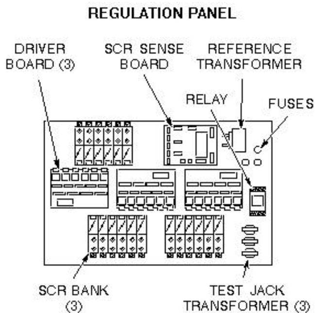
ILLUSTRATION L2750A REG. PANEL COMP. LOCATIONS
