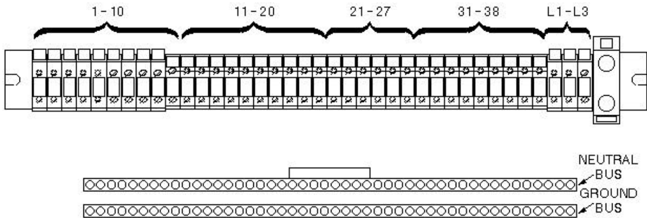
ILLUSTRATION L2745B TB10 (A2) AND BUS BARS MODELS 46-317099P8 THROUGH P22
