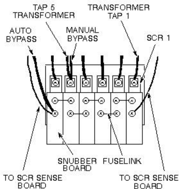
ILLUSTRATION L2752A SCR BANK COMP. LOCATIONS
