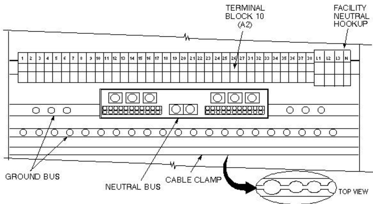
ILLUSTRATION L2741A TB 10 (A2) AND BUS BARS - MODELS 46-317099P1 THRU P4
