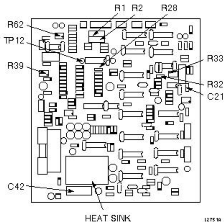
ILLUSTRATION L2751A LOGIC BD COMPONENT LOCATIONS
