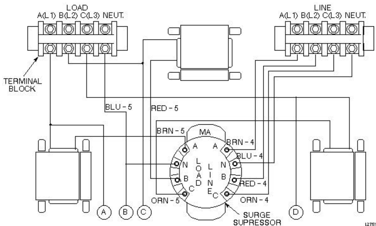
ILLUSTRATION L2755A 50 HZ FILTER COMPONENT LOCATIONS (MODEL 46-317099P2)
